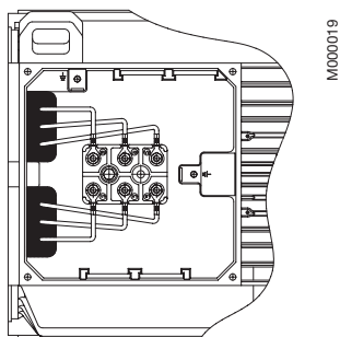
Terminal box size 160-180
