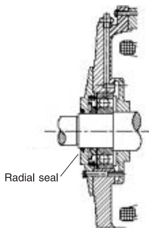
Radial seal (alternative)
