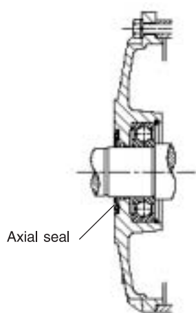
Axial seal
