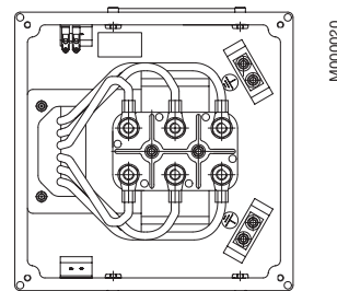
Terminal box size 200-280.
