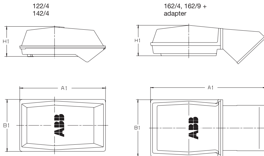
Top-mounted terminal box:
